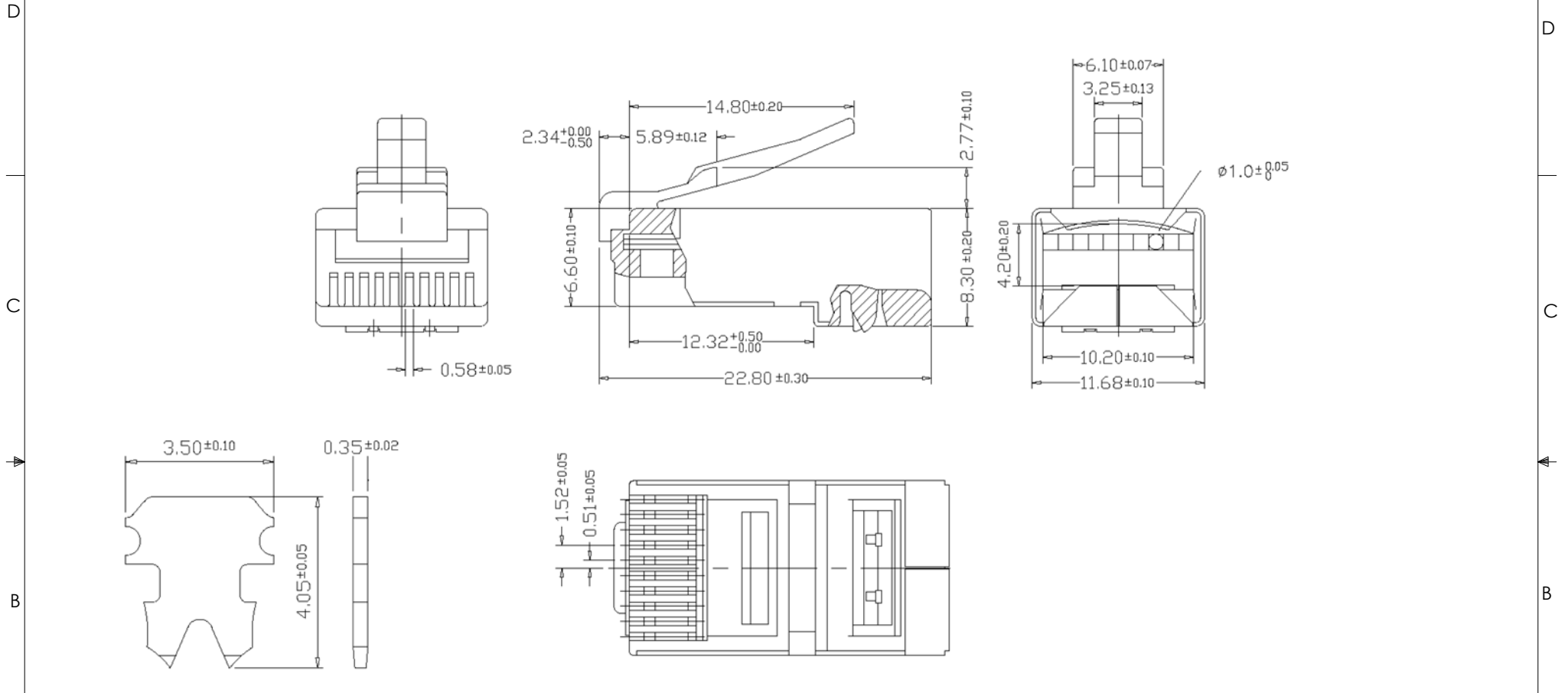
2 PRONG CONTACT FOR STRANDED WIRE
