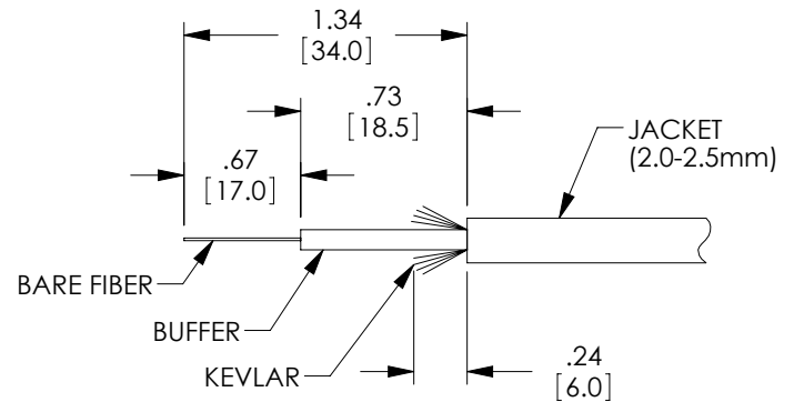
RECOMMENDED STRIPPING DIMENSIONS
